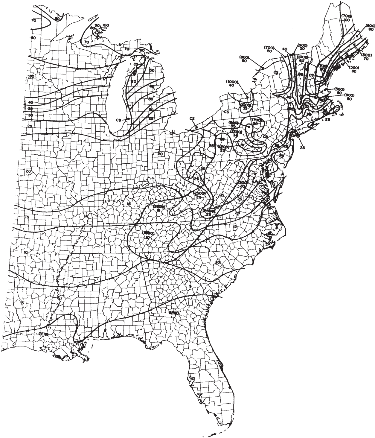
N FIGURE A.3.3.35(b) Ground Snow Loads, p_g , for the United States ( \text{lb}/\text{ft}^2 ). (Source: Reprinted with permission from ASCE/SEI 7.)
